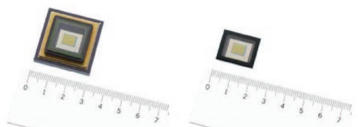
Ceramic PGA package with integrated thermoelectric cooling
