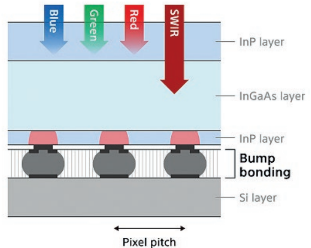
Bump bonding
