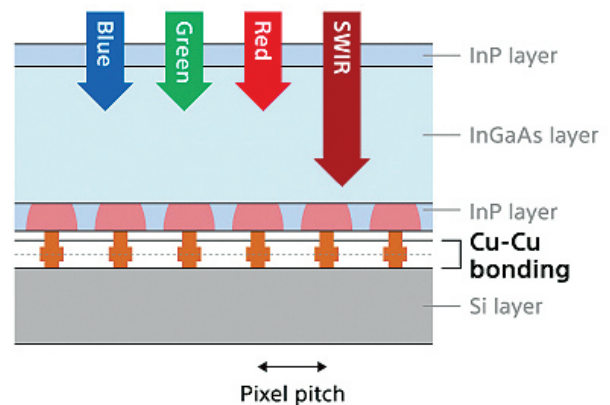
Cu-Cu bonding
