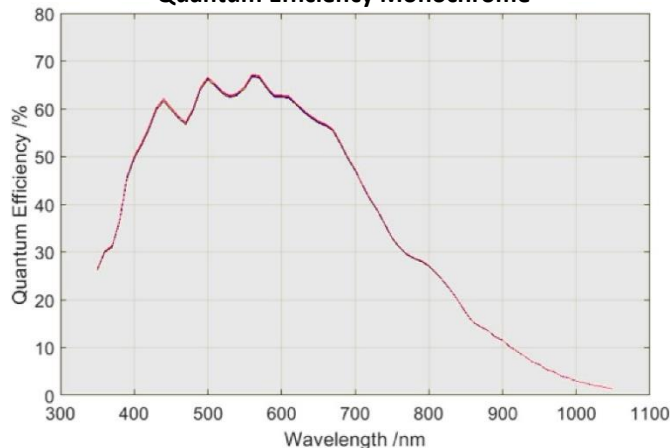
Quantum Efficiency Monochrome
